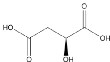
L-malic acid
