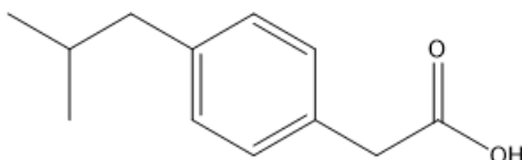
4-isobutylphenylacetic acid
