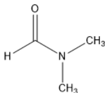
N,N -dimethylformamide
