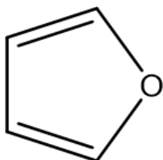
furan
